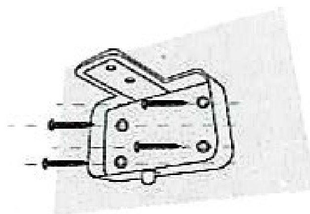
Wall mounted
