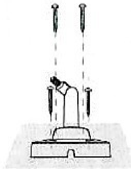
Top mounted
